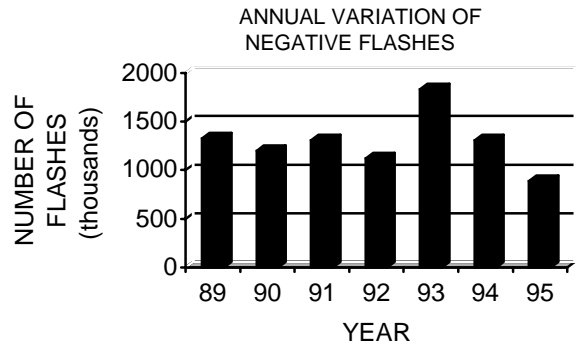
Fig. 4. Annual variation of the number of negative flashes in the region of interest from 1989 to 1995.
