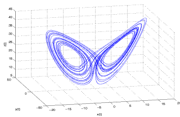
Figure 1: Lorenz system atractor for \sigma=10, \rho=28, \beta=8/3 .
